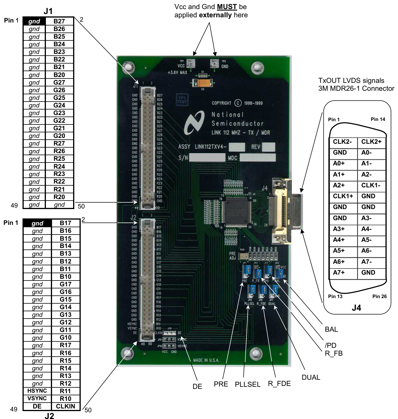
Figure 2. Transmitter Board
